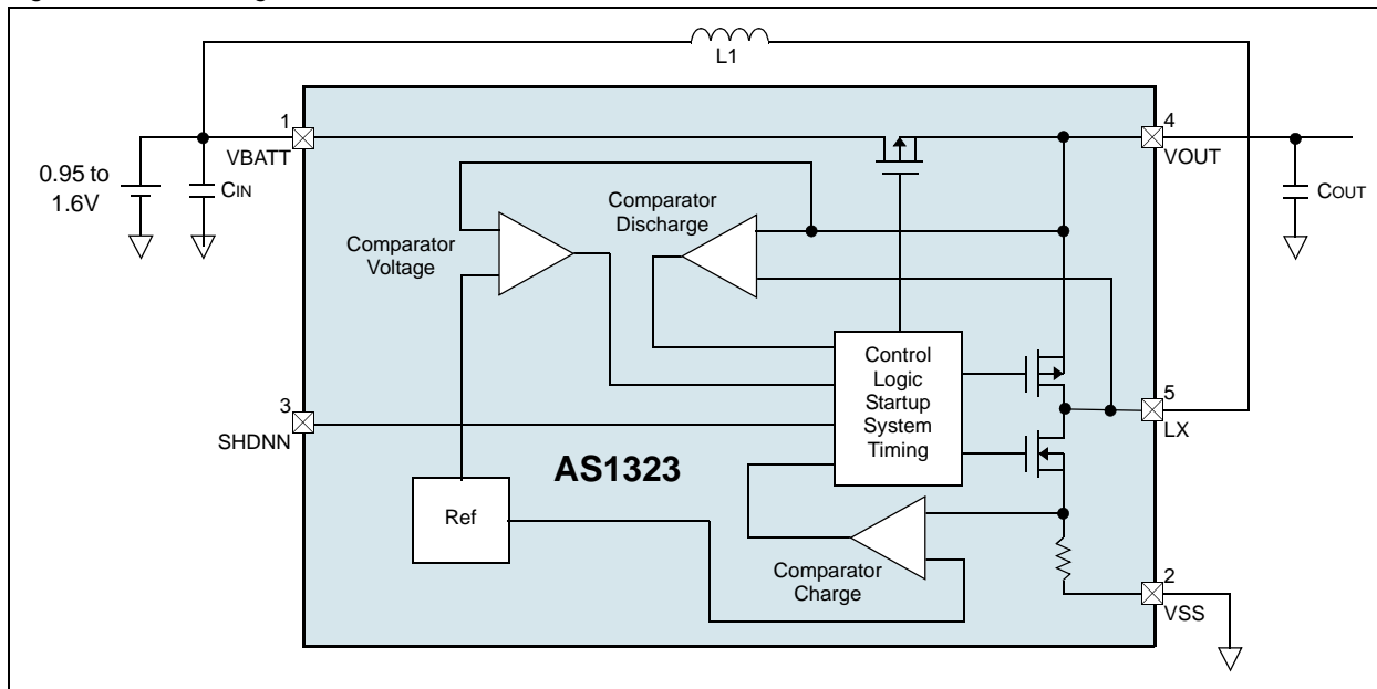
Figure 19. Block Diagram
