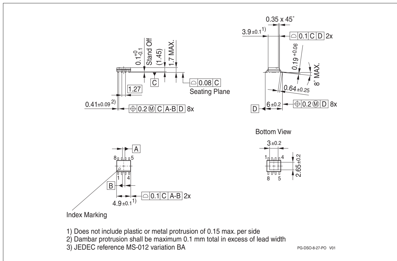
Figure 5 PG-DSO-8 EP
