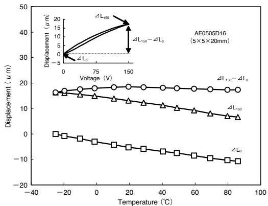
Fig-6 Temperature vs. Displacement
