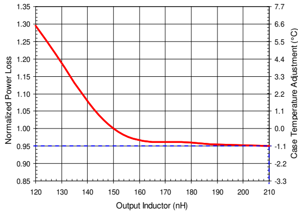
Figure 18 Normalized Power Loss vs. Output Inductor
