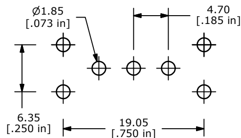
P.C. MOUNTING
