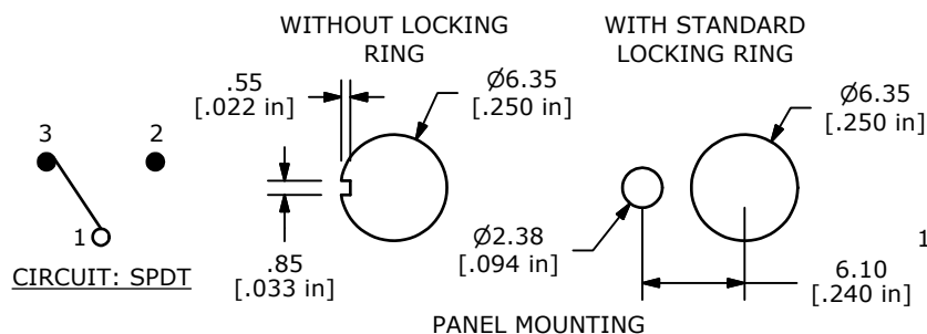
PANEL MOUNTING
