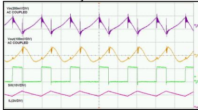
Steady State Test 2A
