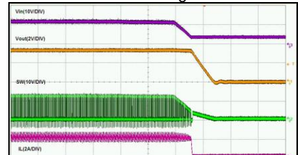
Shutdown Through Vin 2A
