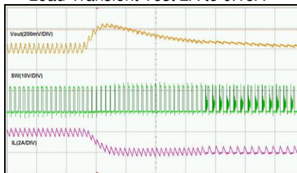
Load Transient Test 2A to 0.15A
