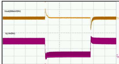
Load Transient Test 0.15 to 2A
