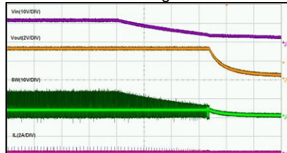
Shutdown Through Vin no load
