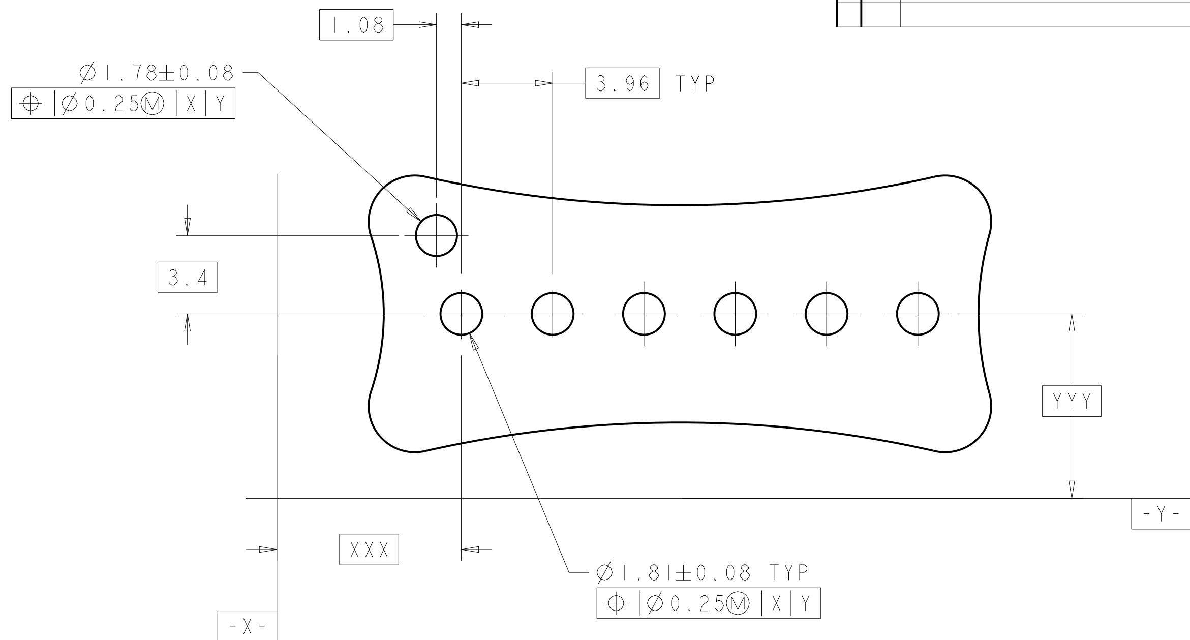
RECOMMENDED PCB LAYOUT SCALE 6:1
