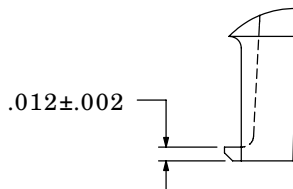
DETAIL A SCALE= 6X
