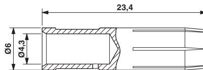
Dimensional drawing
