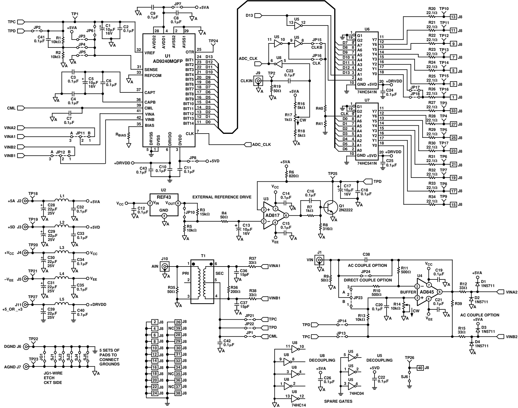
Figure 55. Evaluation Board Schematic
