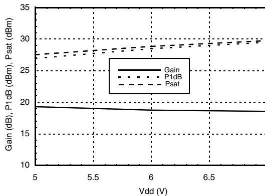
Gain & Power vs. Supply Voltage @ 20 GHz
