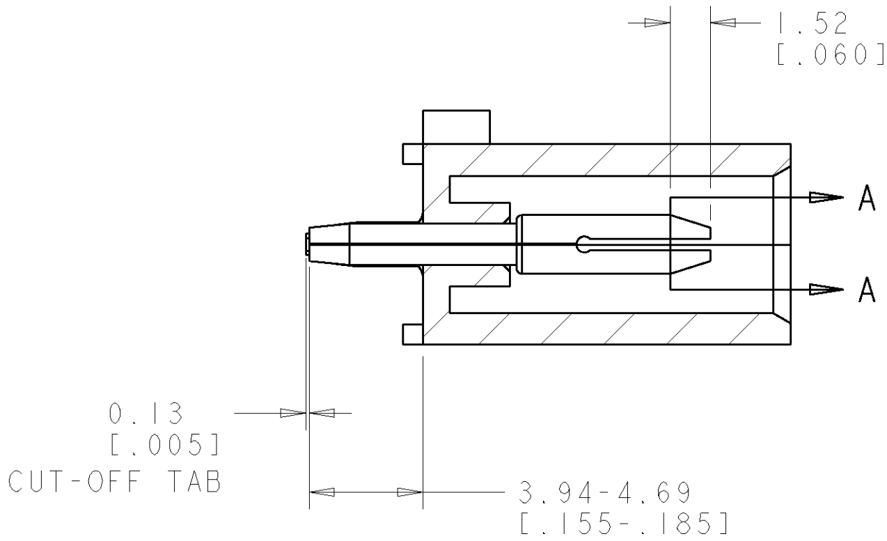
SECTION B-B
